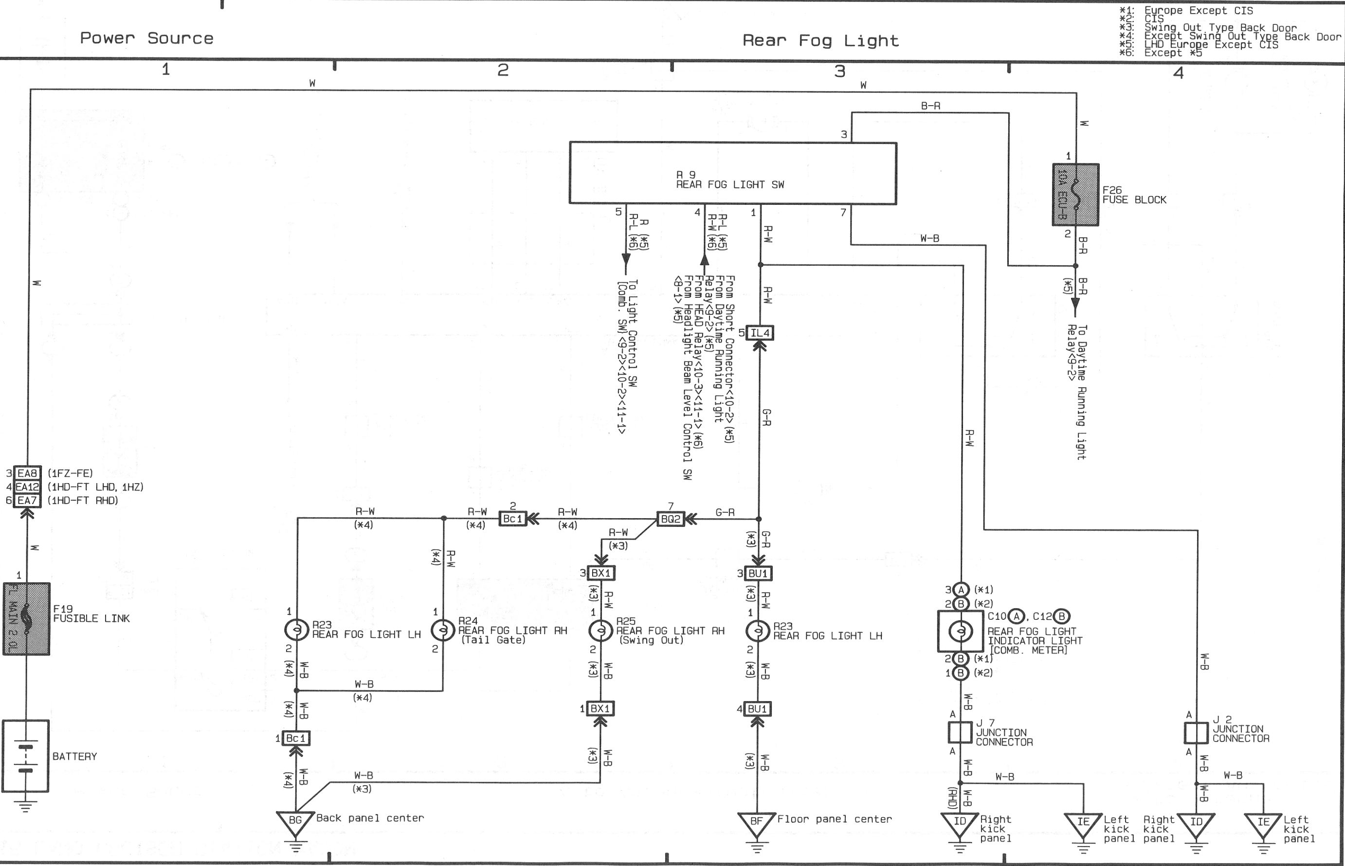
G OVERALL ELECTRICAL WIRING DIAGRAM
